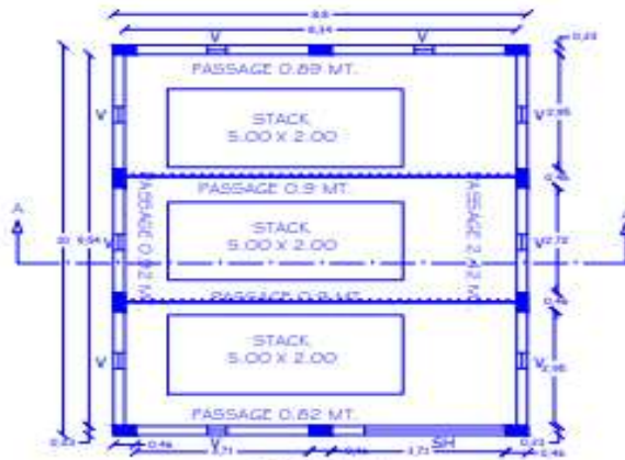
GODOWN PLAN SCALE 1:100
